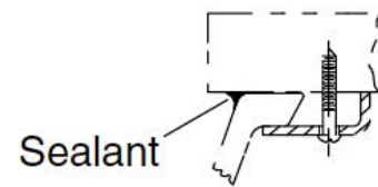
Wood Installation
