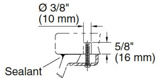
Standard Installation:
